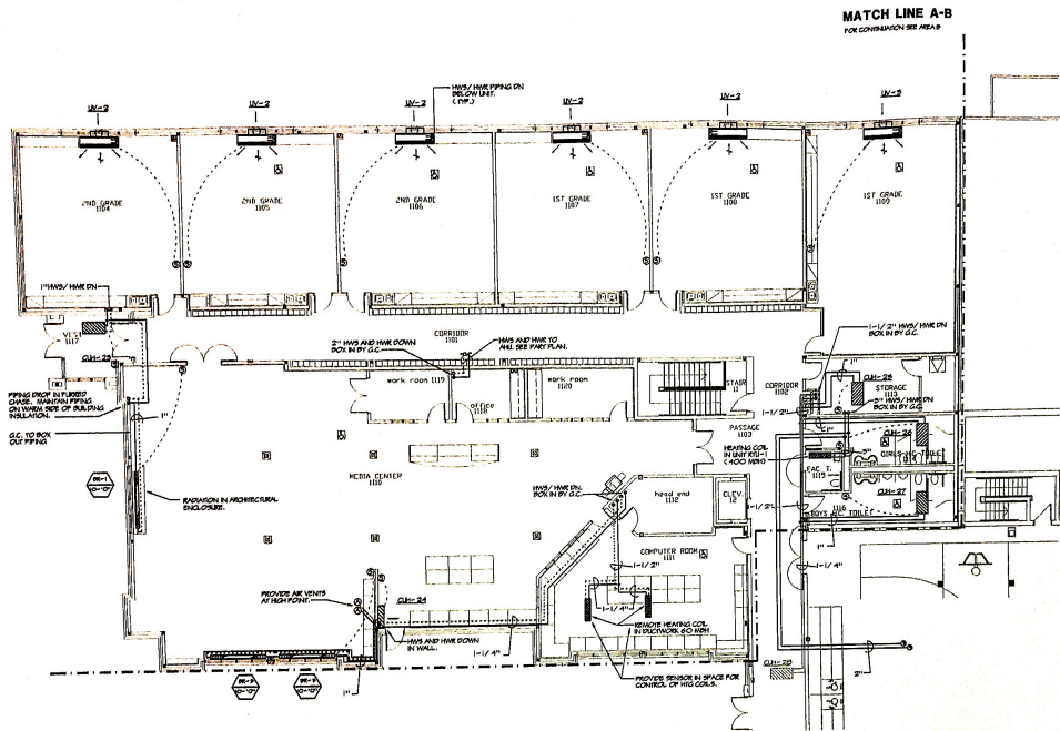
1 HEATING MAIN LEVEL FLOOR PLAN - AREA A SCALE: 1/8" = 1'-0" 12/22/88 1. REFER TO SCHEDULES AND DETAIL DRAWINGS.
