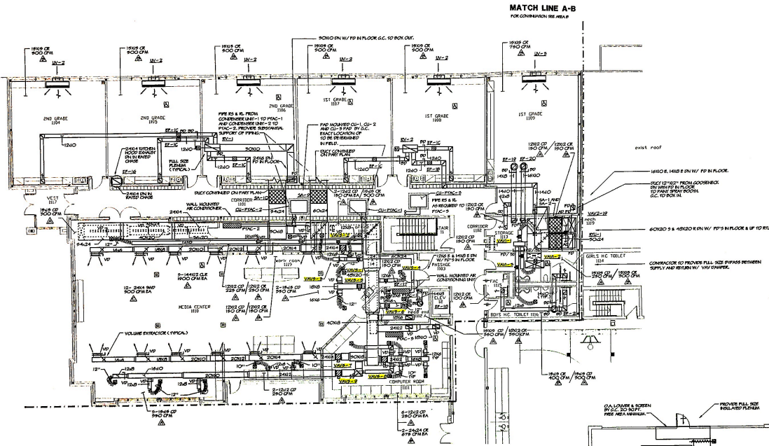
1 MECHANICAL MAIN LEVEL FLOOR PLAN - AREA A SCALE: 1/8" = 1'-0" 1. REFER TO SCHEDULES AND DETAIL DRAWINGS.
