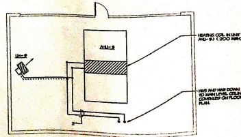
2 HEATING PART PLAN AIR HANDLING UNIT ROOM SCALE: 1/8" = 1'-0" 12/22/88 1. REFER TO SCHEDULES AND DETAIL DRAWINGS.
