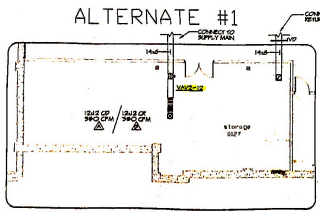
2 MECHANICAL LOWER LEVEL ALTERNATE - AREA A SCALE 1/8" = 1'-0" 1. REFER TO SCHEDULES AND DETAIL DRAWINGS.
