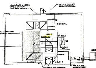
2 MECHANICAL PART PLAN - PENT HOUSE SCALE: 1/4" = 1'-0" 1. REFER TO SCHEDULES AND DETAIL DRAWINGS. 2. REFER TO FLOOR PLAN.
