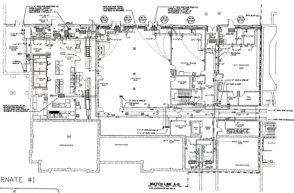
1 HEATING LOWER LEVEL FLOOR PLAN - AREA A SCALE: 1/8" = 1'-0" 1. REFER TO SCHEDULES AND DETAIL DRAWINGS.
