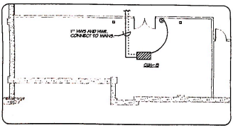
1 HEATING LOWER LEVEL FLOOR PLAN - ALTERNATE #1 - AREA A SCALE: 1/8" = 1'-0" 1. REFER TO SCHEDULES AND DETAIL DRAWINGS.
