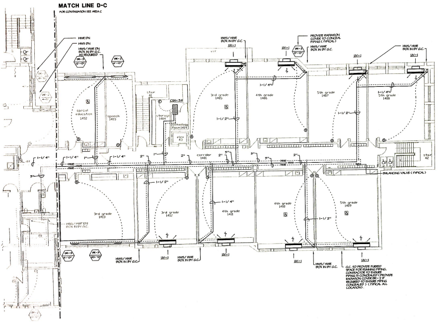
1 HEATING MAIN LEVEL FLOOR PLAN - AREA D
